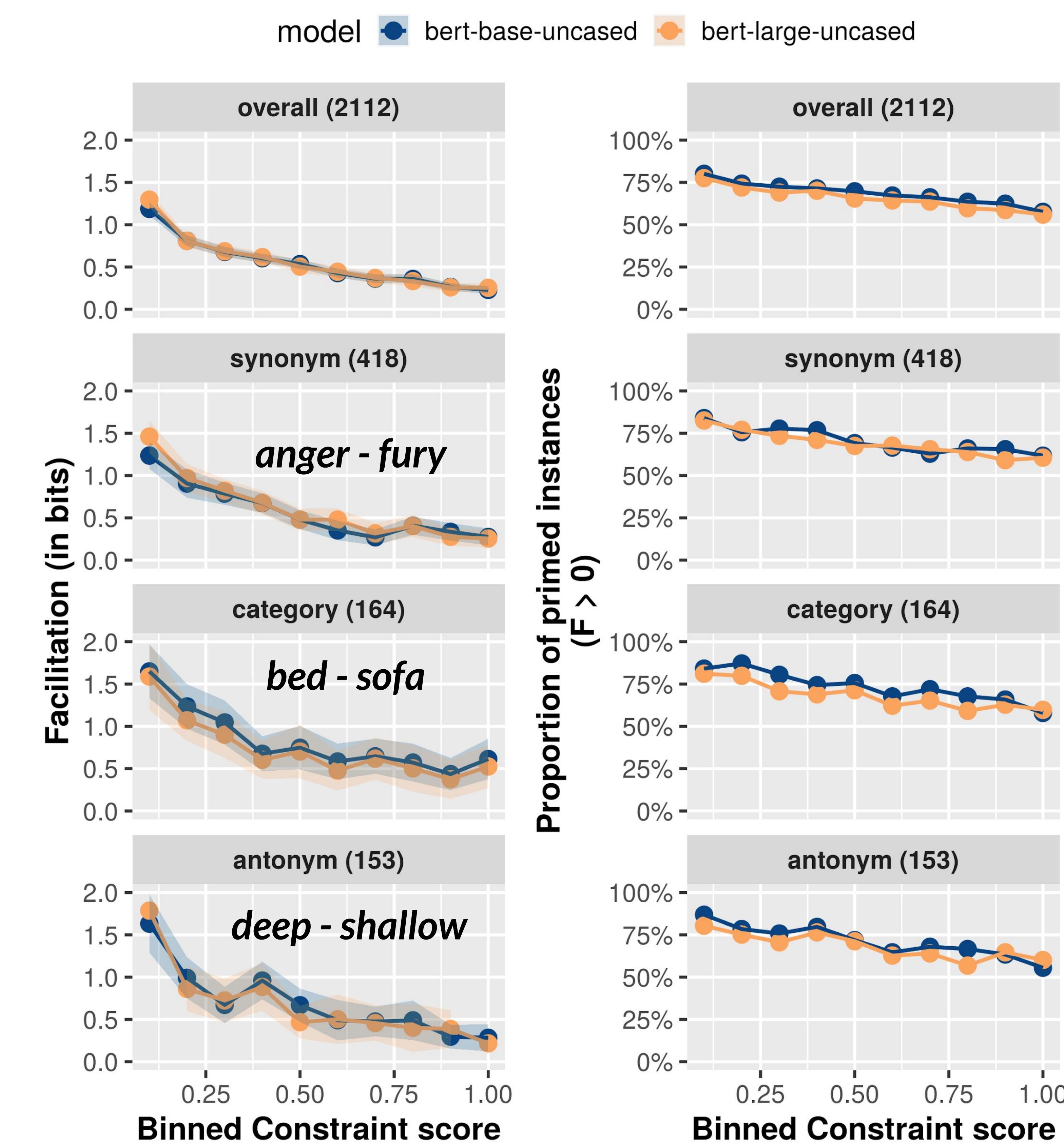
Figure 1: Facilitations (left) and proportion of primed instances (right) across the top-3 lexical relations, along with overall results (first row). The x-axis denotes binned constraint scores (0.1-1.0)
